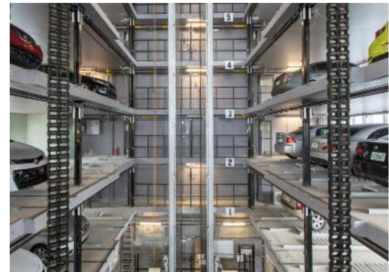
High Density Parking System (Shuttle Type)
